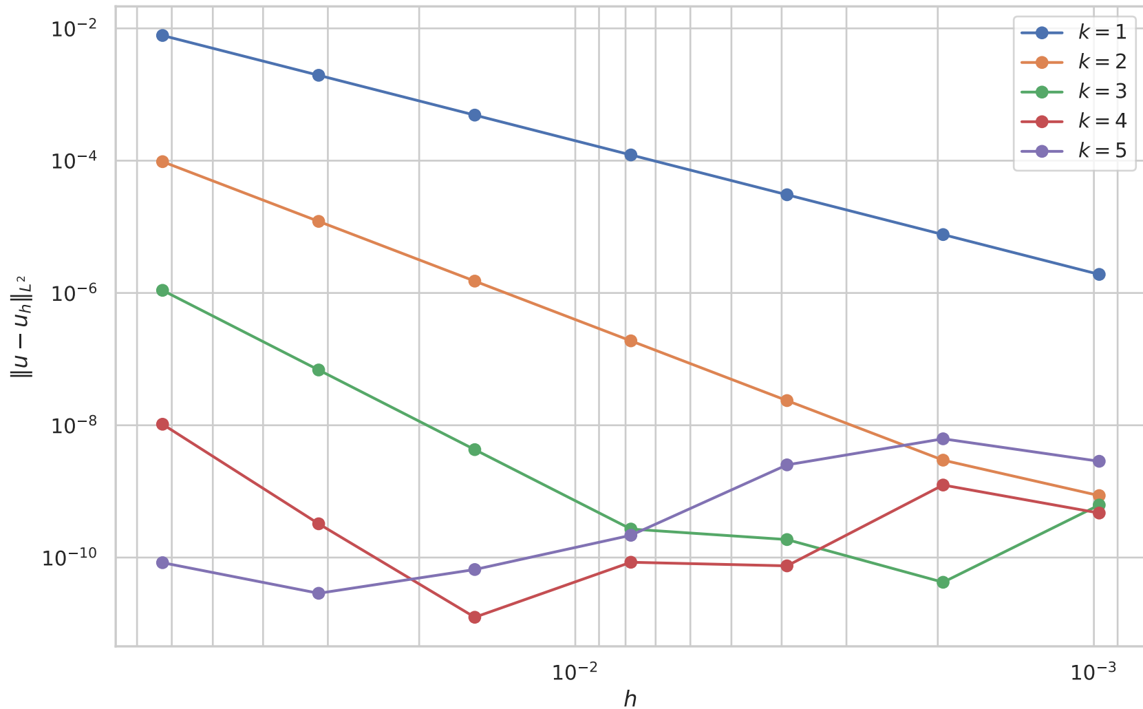
Item (h): erro de u_h com \delta_1 = -1/2 , \delta_2 = 1/2 e \beta = 0
