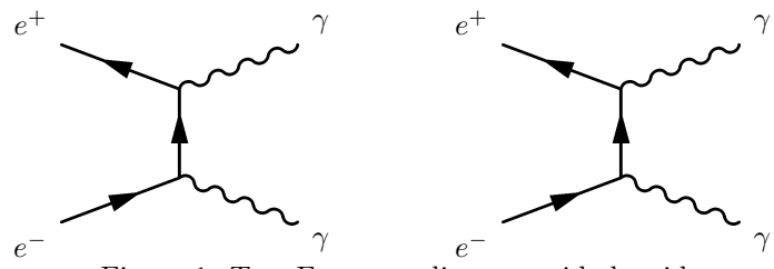
Figure 1: Two Feynman diagrams side-by-side
