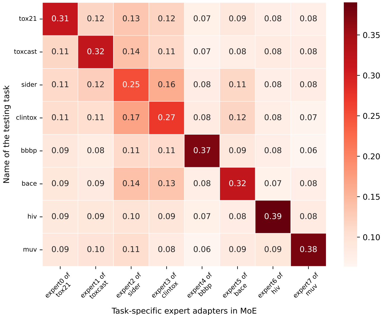
MoE Weights Heatmap
