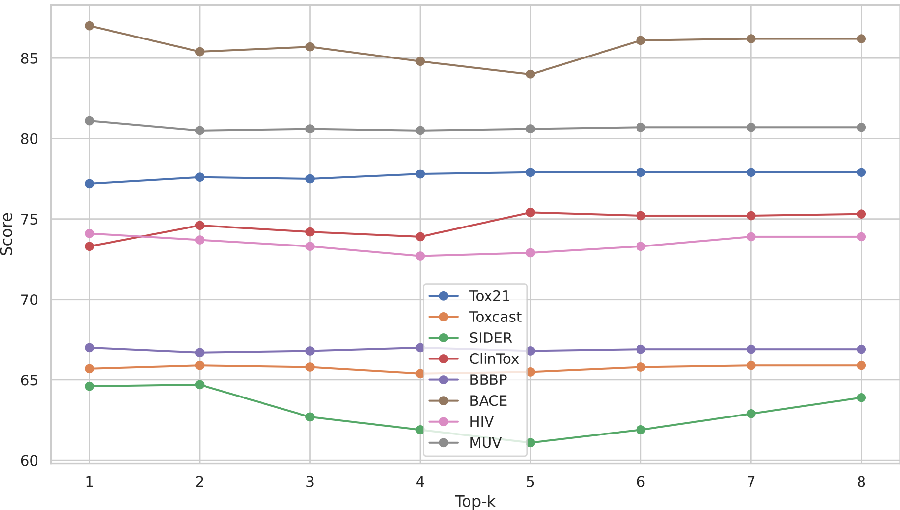
Performance across Different Top-k in MoE
