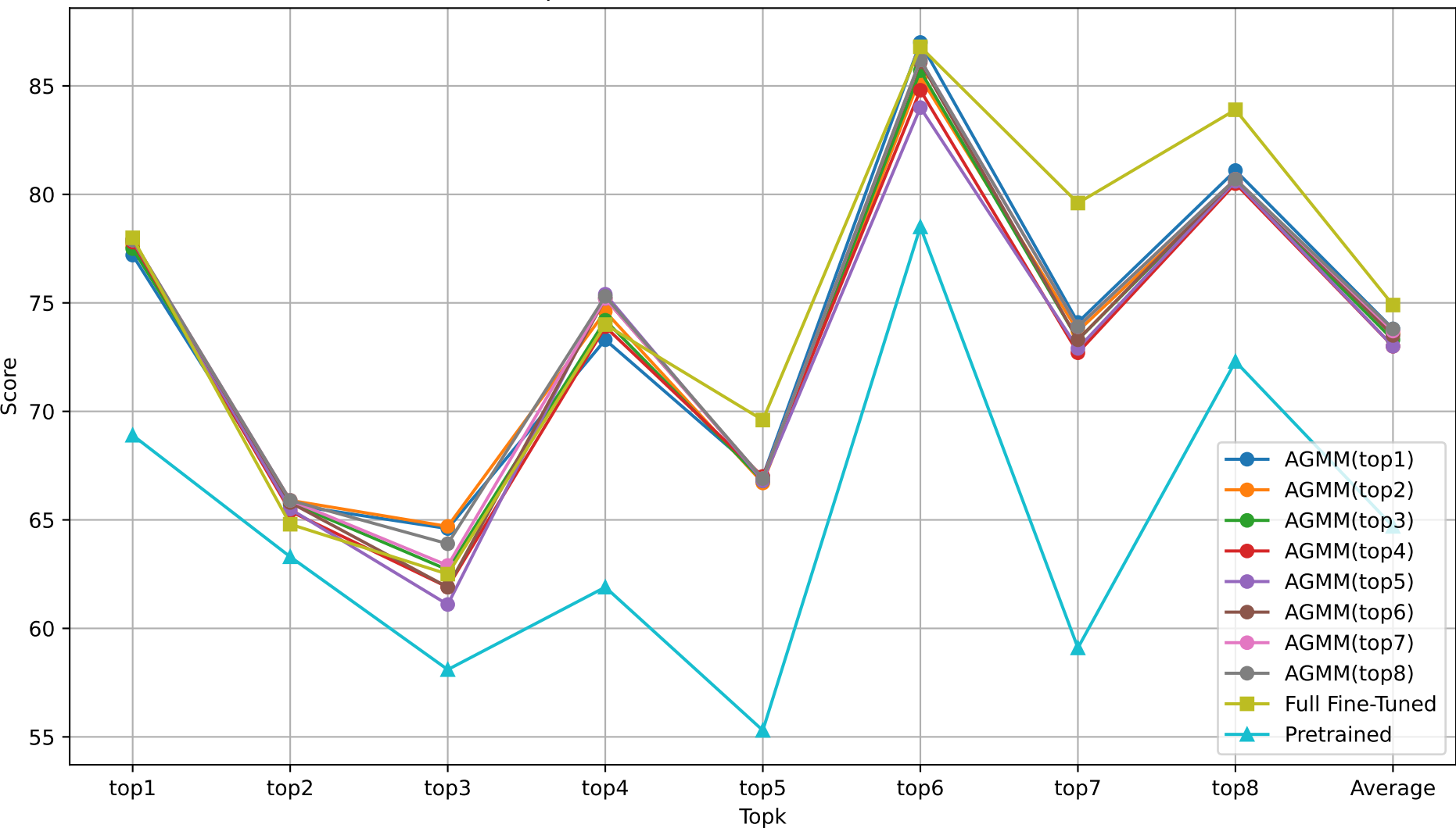
Topk Performance of Different Methods
