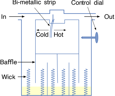
Tec 5 Schematic
