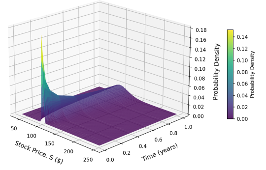
Fig. 3. PDF evolution from Monte Carlo particle data.
