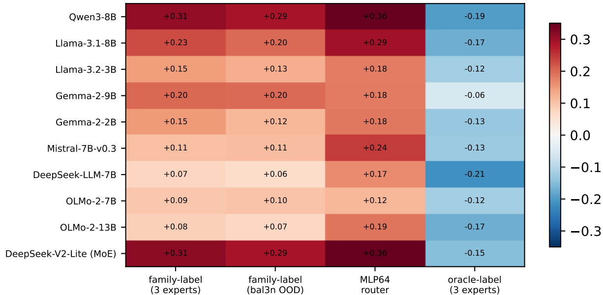
Decision-interface sensitivity ( \Delta BA, pretrained – random)
