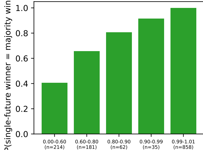
label flips concentrate in near-ties
