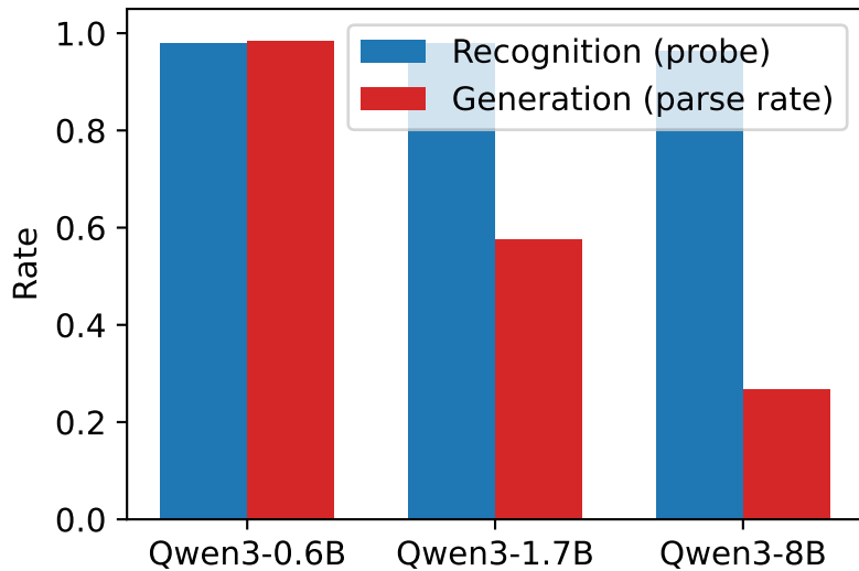
Frozen: recognize vs. generate
