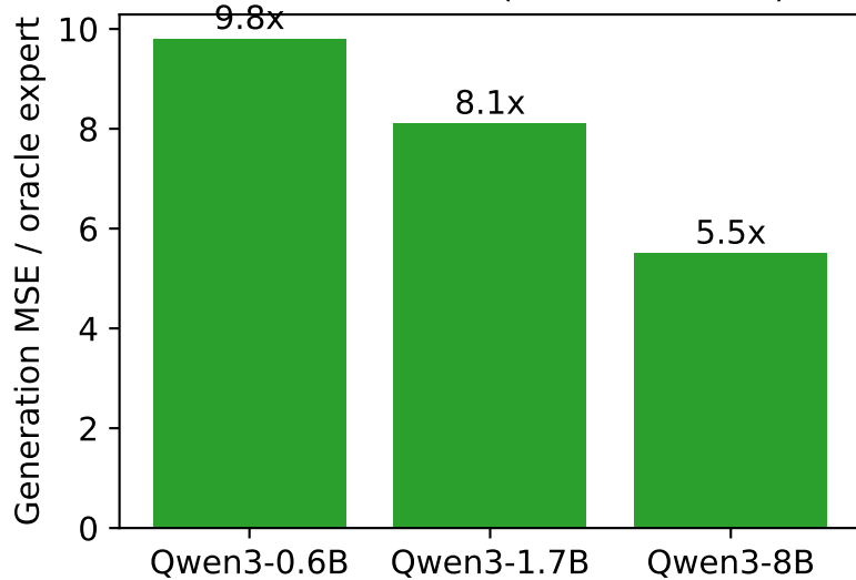
Generation error (same windows)
