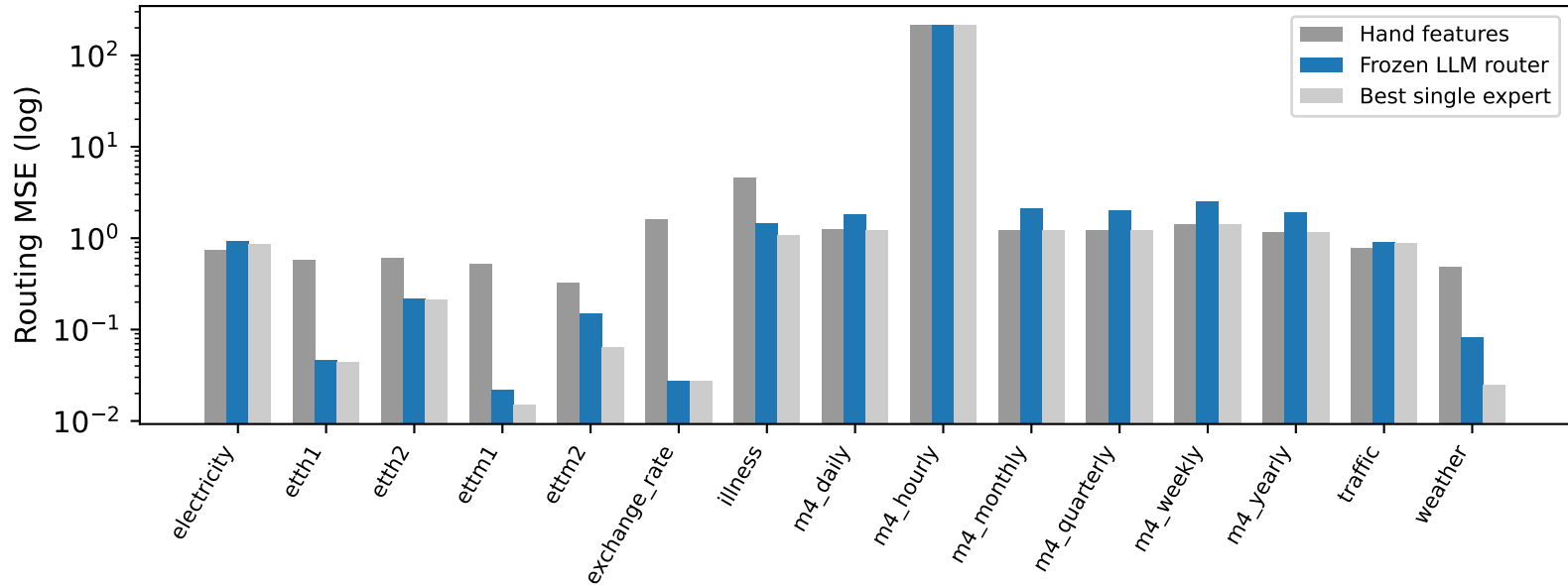
Zero-shot routing on 15 real datasets (Qwen3-8B)
