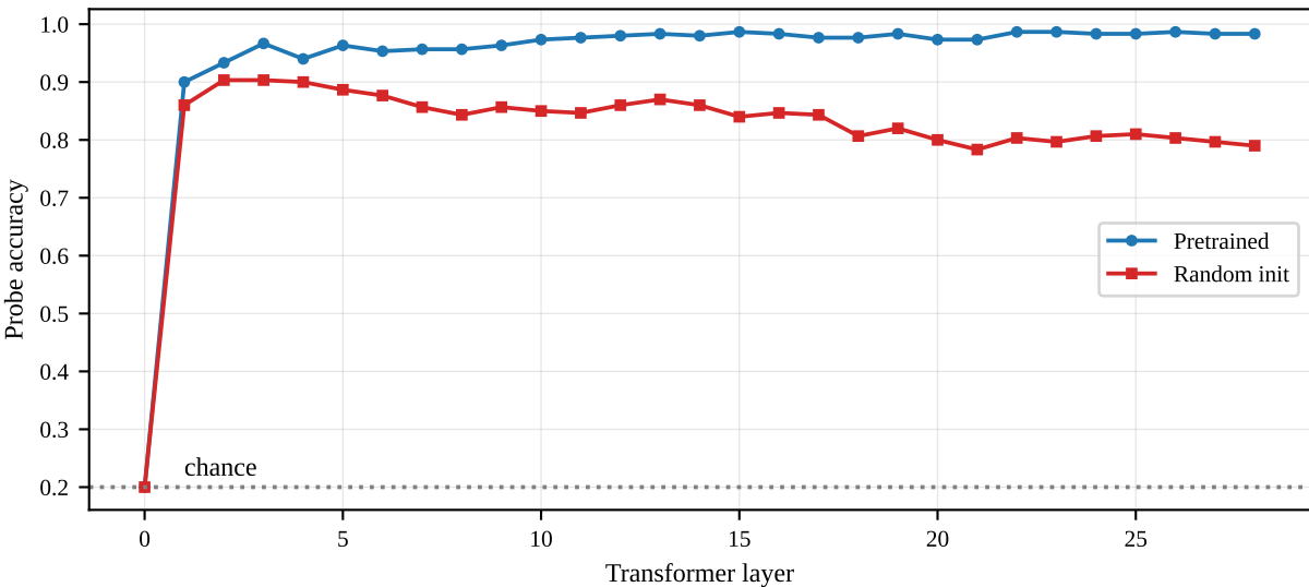
Layer-wise temporal-structure recognition (Qwen3-0.6B)
