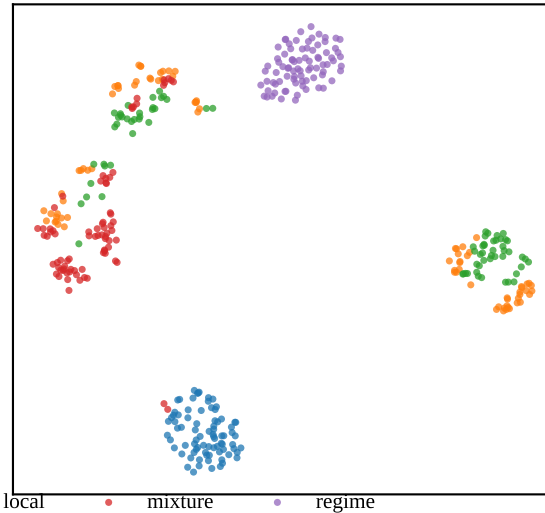
Pretrained – t-SNE
