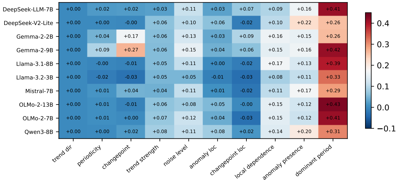
Figure A — Temporal abstraction map: pretrained – random probe gain (final layer)
