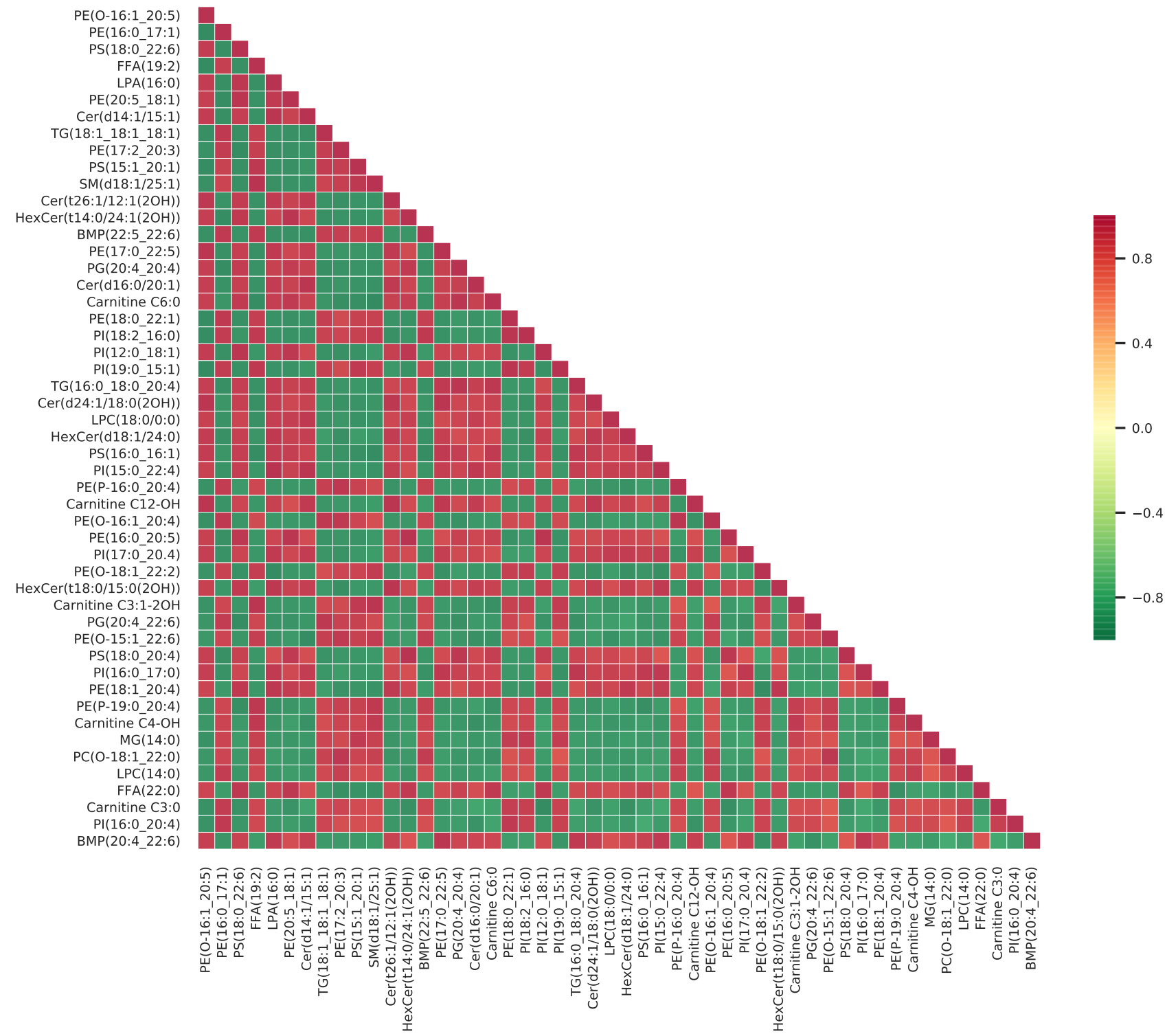
Pearson Correlation Plot of A_vs_B
