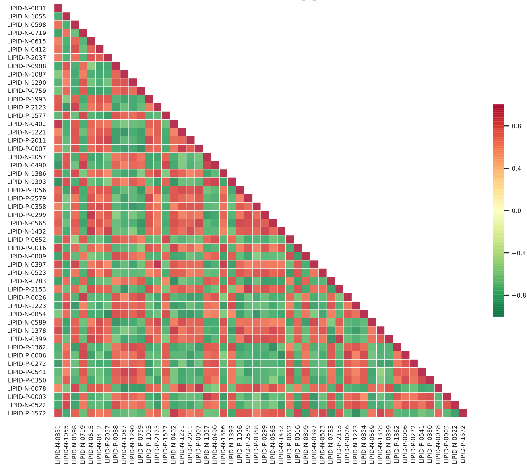
Spearman Correlation Plot of A_vs_B
