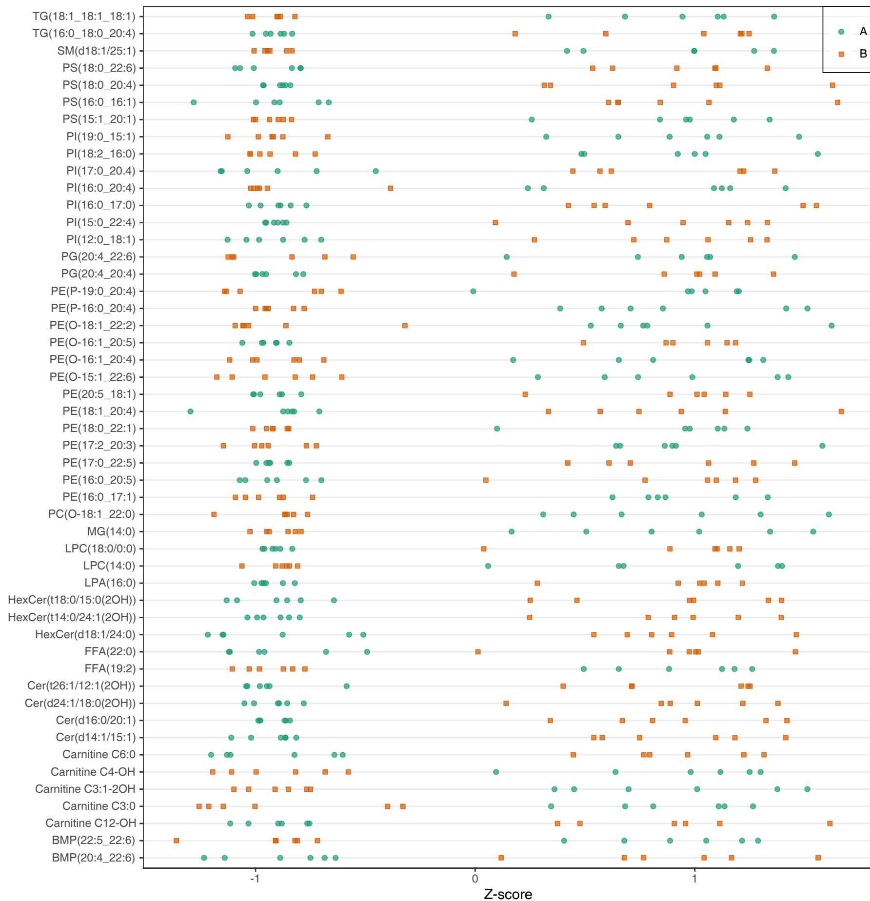
A_vs_B Z-score Plot
