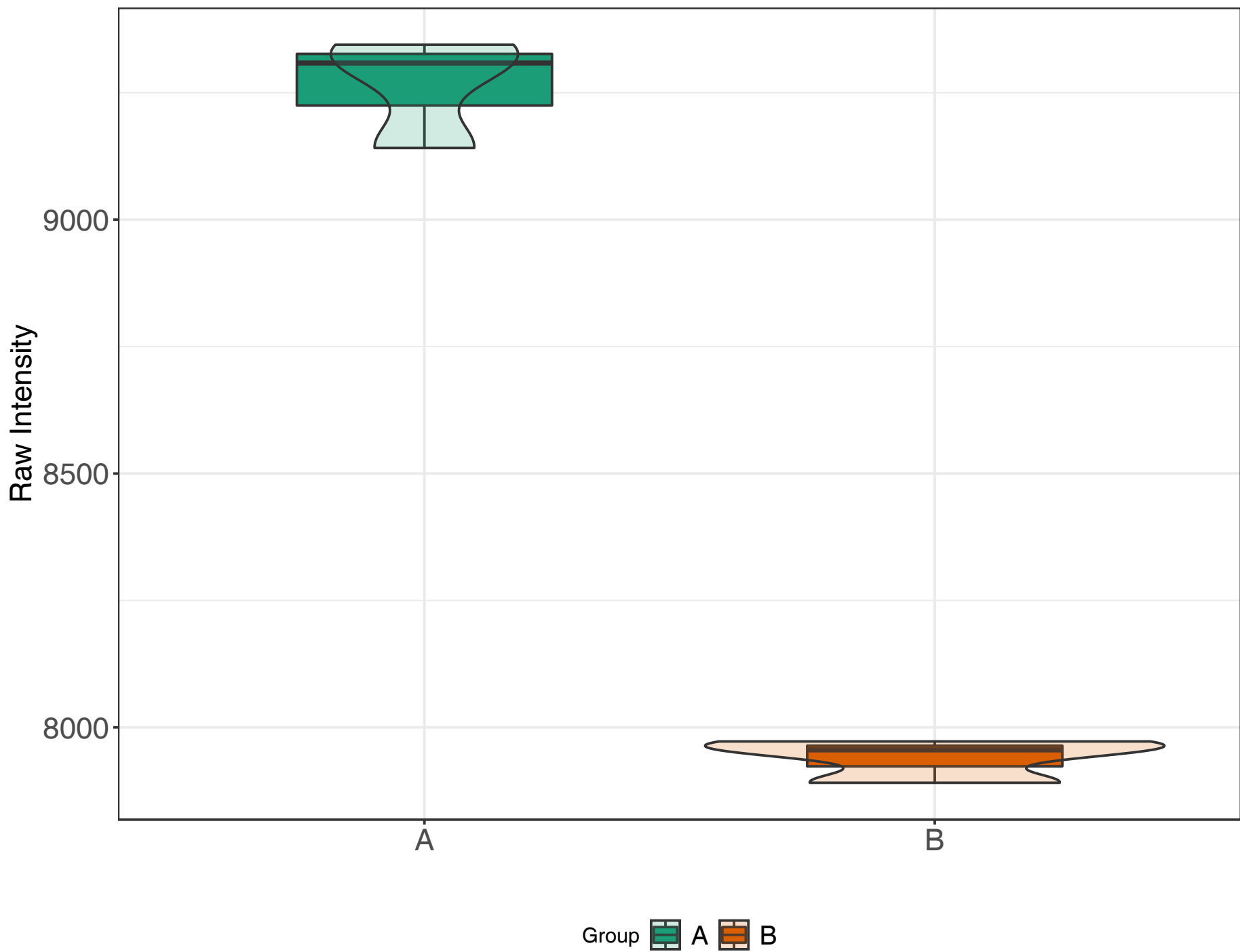
6- \{[3-(3,4\text{-dimethoxyphenyl})-7\text{-methoxy-8-methyl-4-oxo-4H-chromen-5-yl]oxy}\} -3,4,5-trihydroxyoxane-2-carboxylic acid
