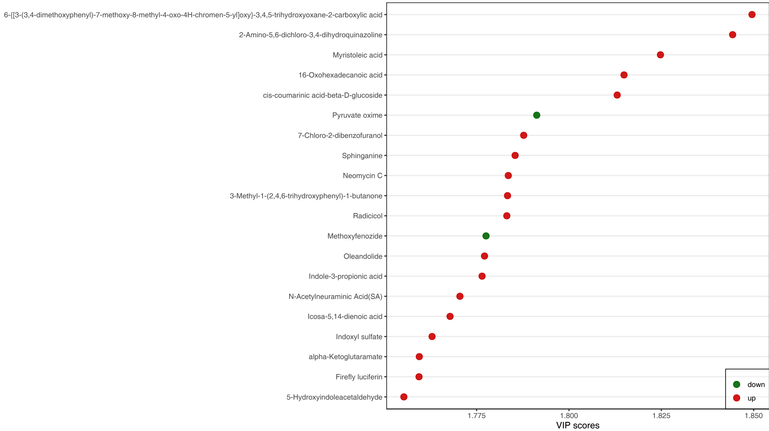
A_vs_B VIP score Plot
