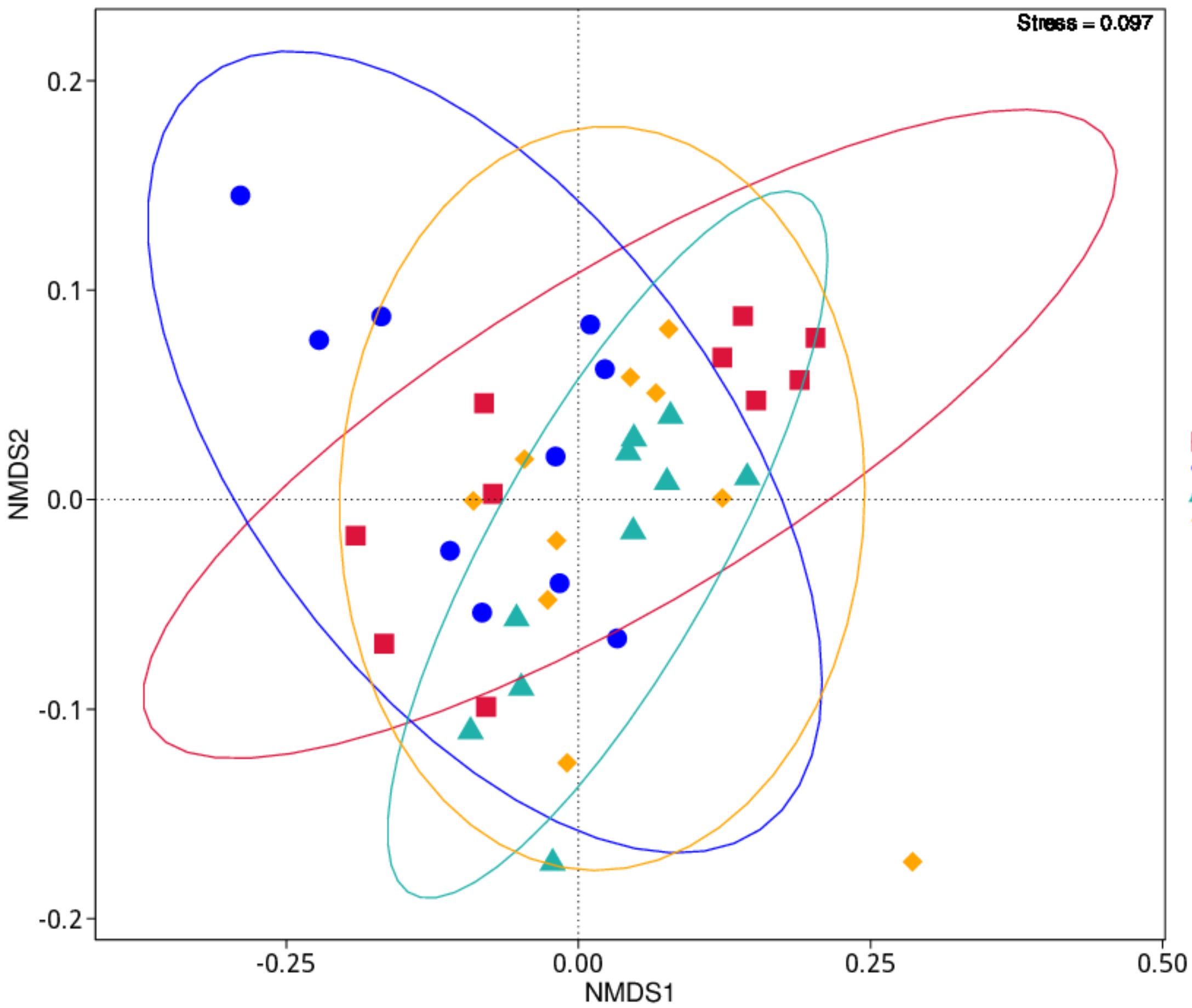
NMDS Plot
