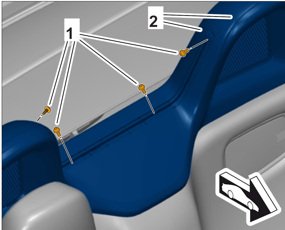
翻滚防护杆饰板的紧固螺钉
