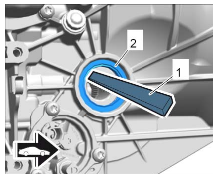
撬出密封环
