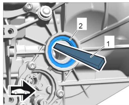
撬出密封环
