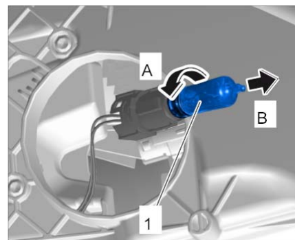
拆卸灯泡
