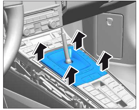
拆卸选档杆罩
