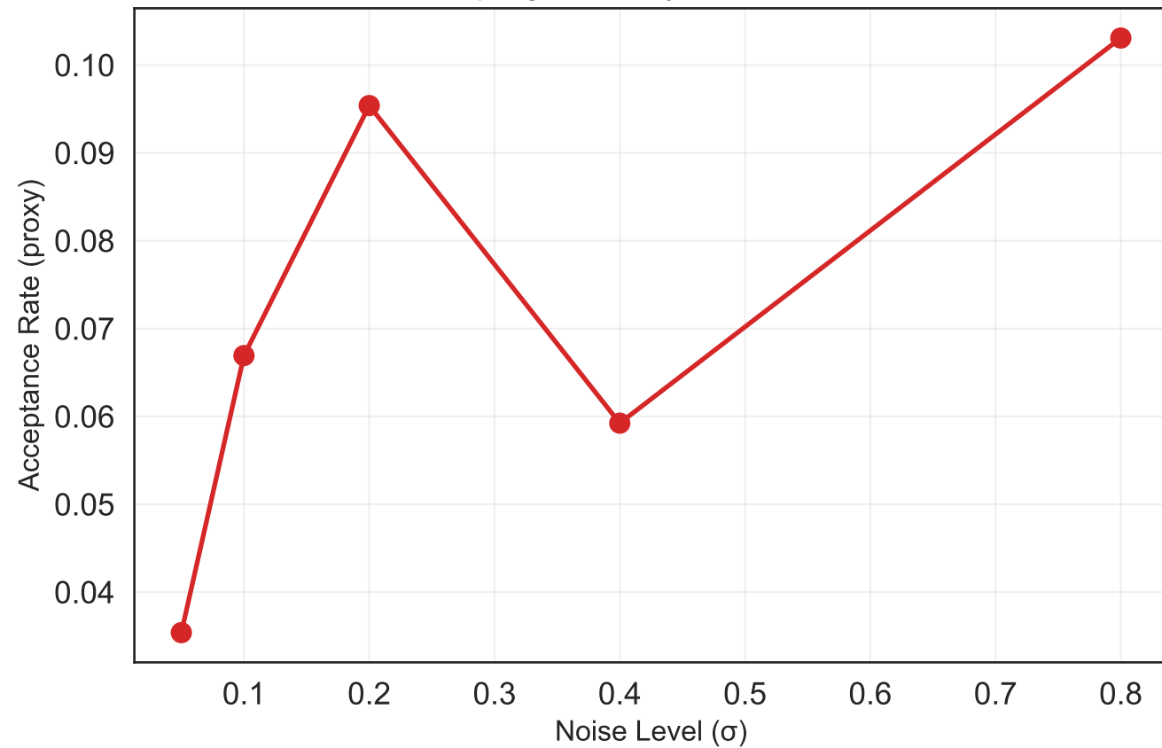
Sampling Efficiency vs Noise Level
