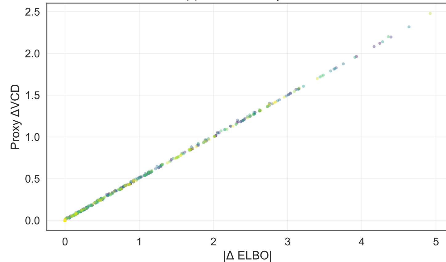
(c) ELBO vs Proxy VCD
