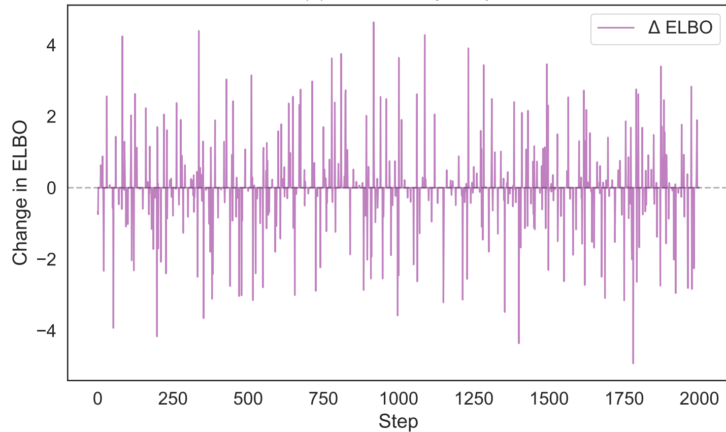
(a) \Delta ELBO Trajectory
