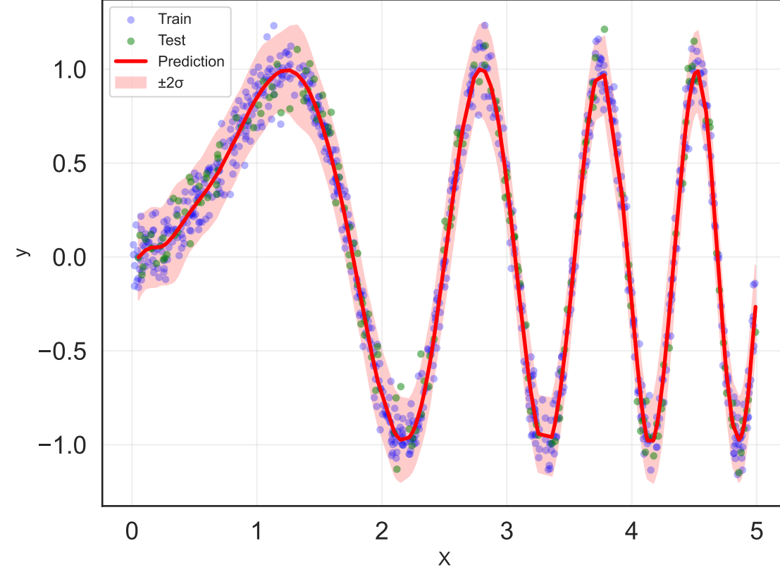
Matern32 RMSE=0.100, NLPD=-0.875
