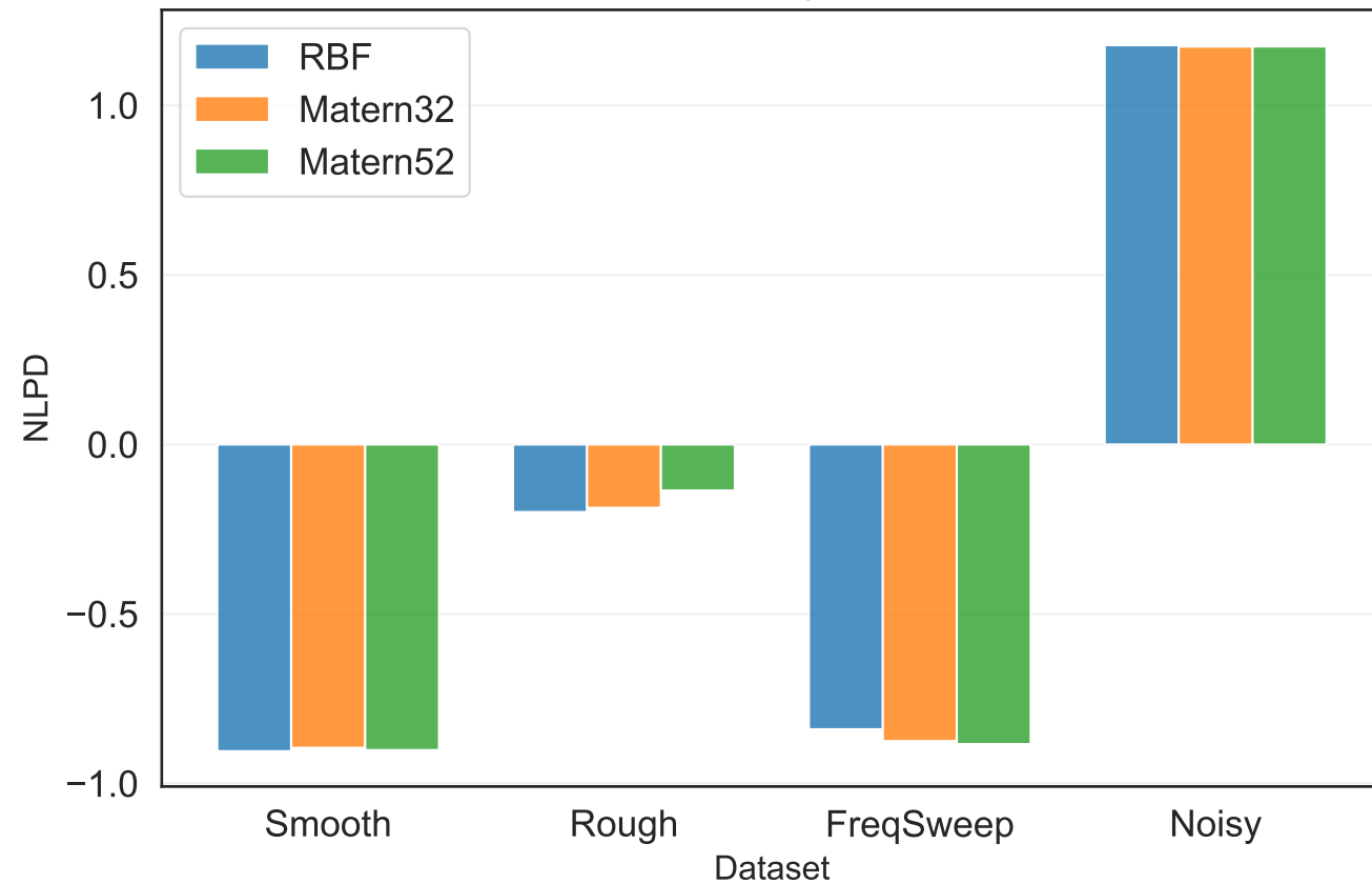
NLPD Comparison
