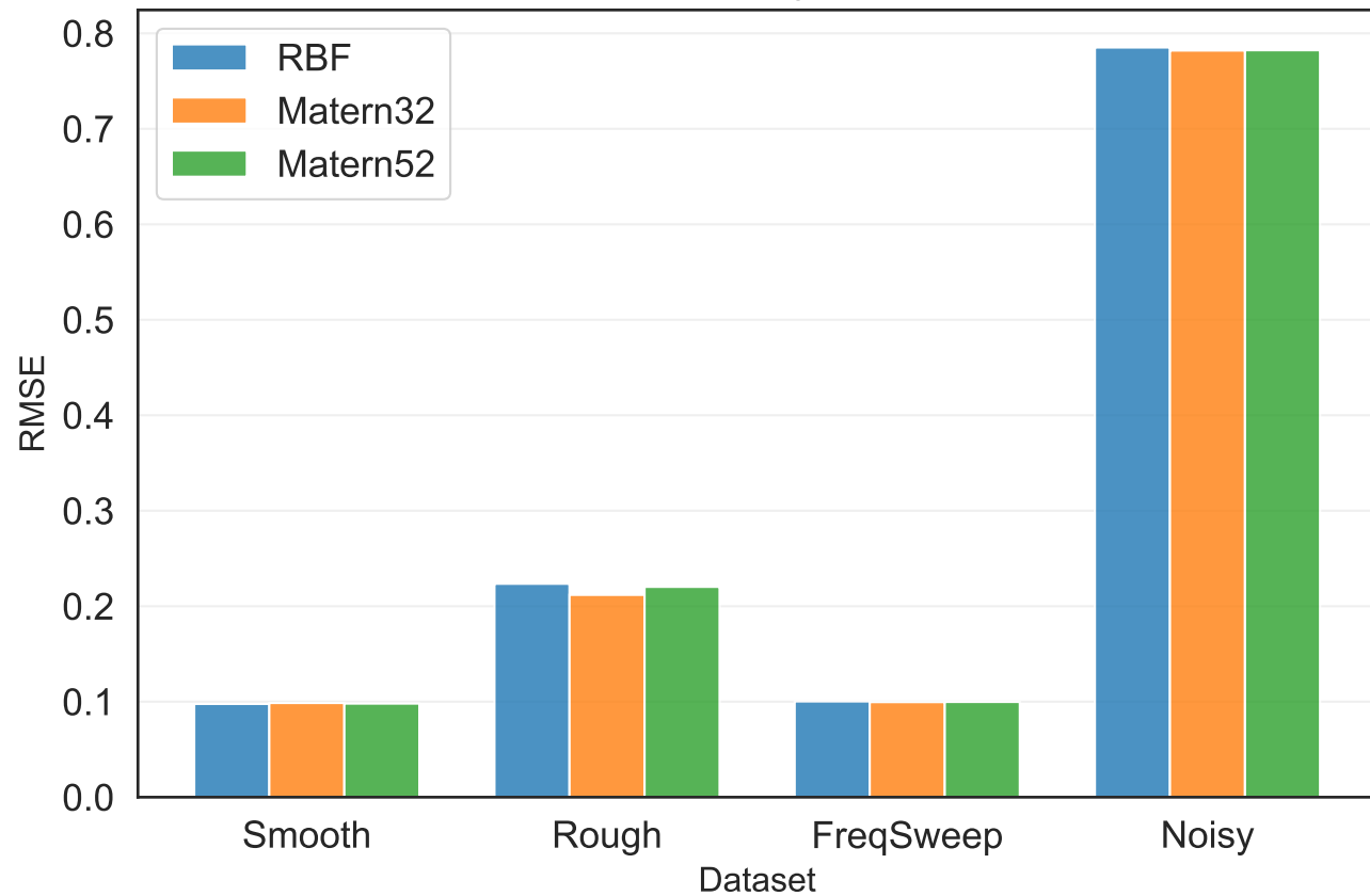
RMSE Comparison
