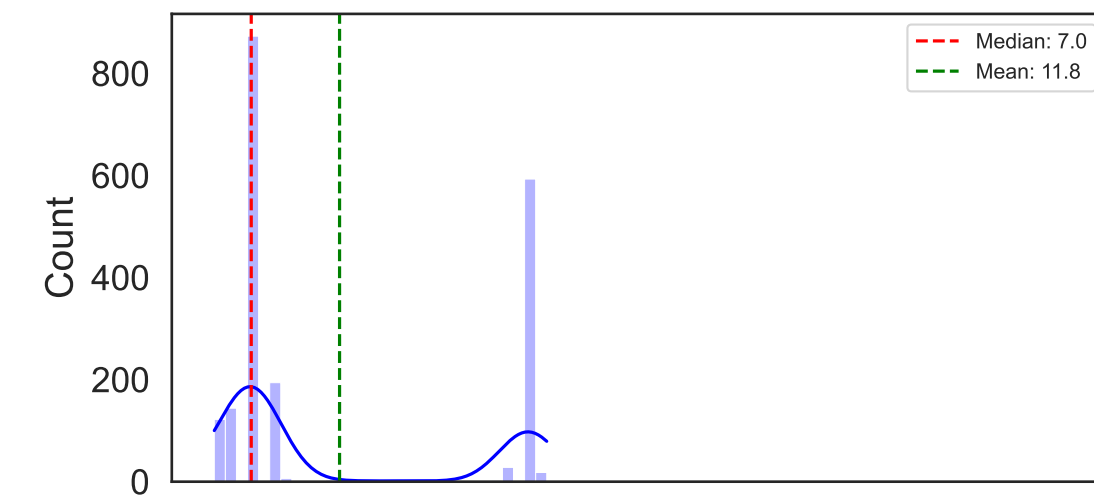
Count
