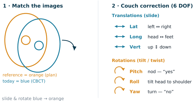
Figure 6.2 — Matching today's image (blue) to the planning image (orange) tells the system how far off the patient is; the couch then corrects in up to six degrees of freedom — three translations (Lat, Long, Vert) and three rotations (pitch, roll, yaw).
