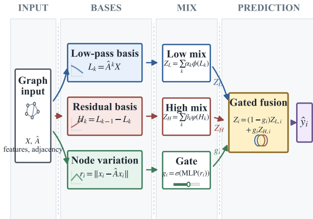
Figure 2: HARP-GNN internal residual polynomial block. HARP-Select uses this self-loop expert as one branch and pairs it with an ego-separated no-self version of the same residual filtering idea.
