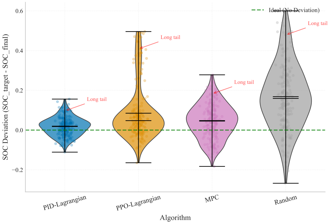
User Satisfaction: SOC Deviation Distribution
