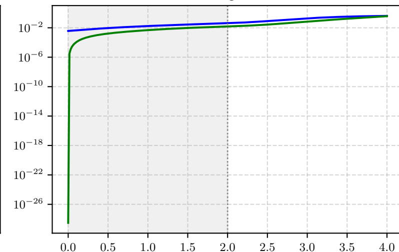
Burgers PDE
