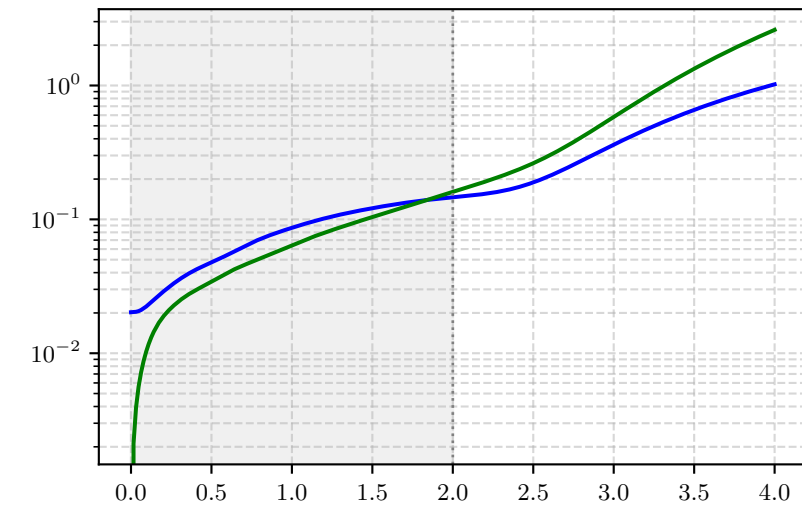
2D Allen-Cahn PDE
