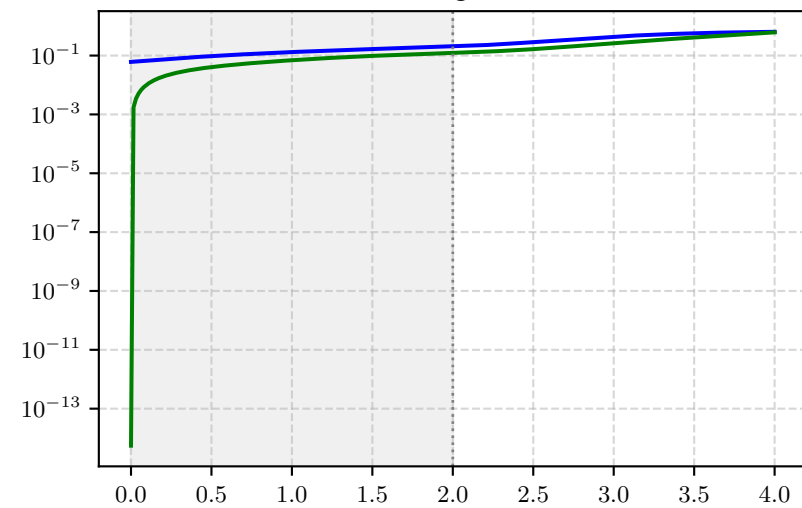
Burgers PDE
