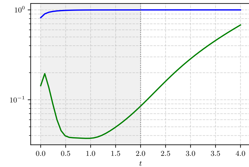
2D Allen-Cahn PDE
