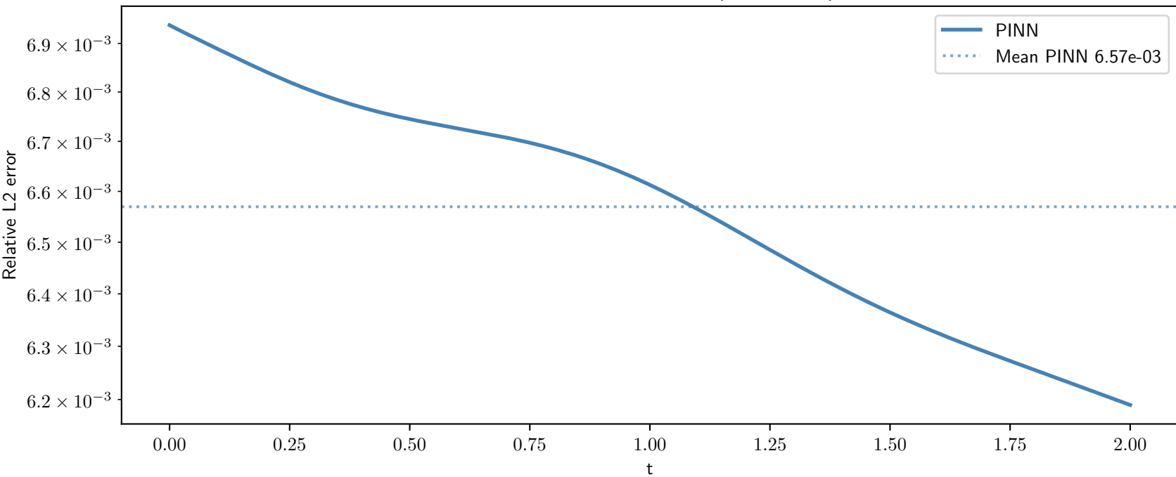
Relative L2 error over time ( \kappa = 0.9132 )
