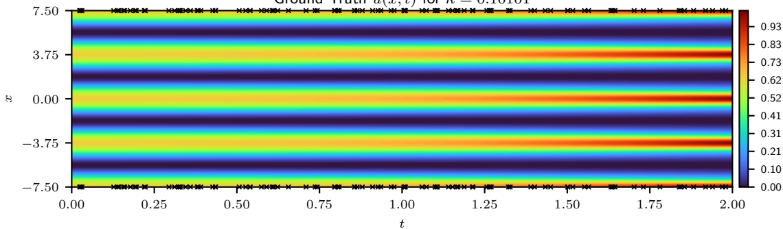
Ground Truth u(x, t) for \kappa = 0.10101
