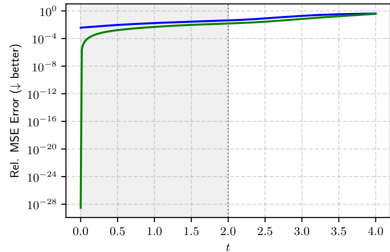
Burgers PDE ( \kappa = 0.028 )
