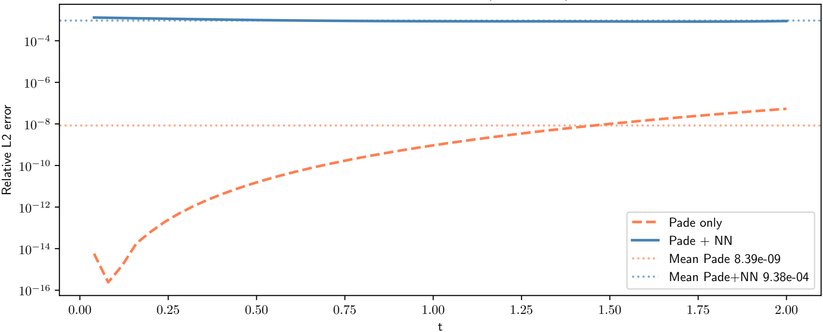
Relative L2 error over time ( \kappa = 0.0110 )
