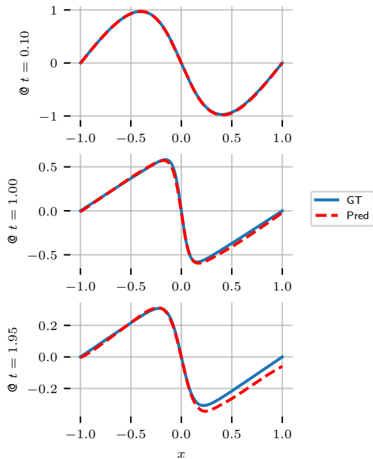
Comparison at Selected Time Points
