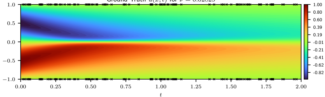
Ground Truth u(x, t) for \nu = 0.02829
