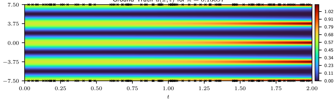
Ground Truth u(x, t) for \kappa = 0.13697
