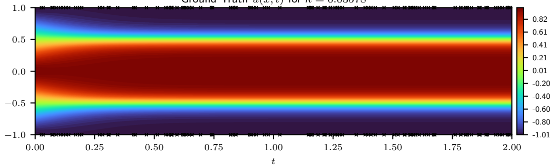
Ground Truth u(x, t) for \kappa = 0.03578
