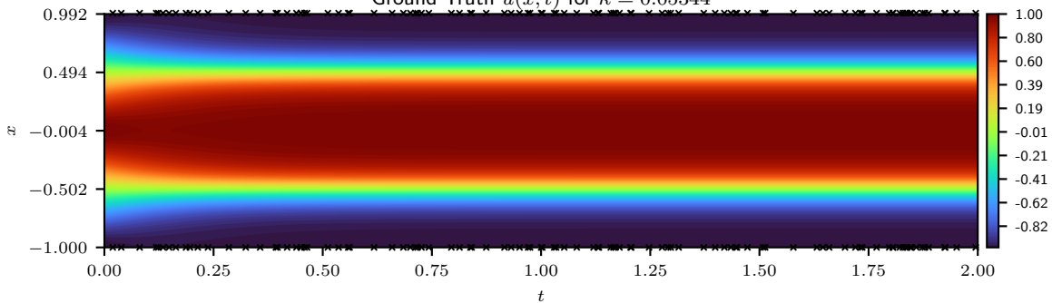
Ground Truth u(x, t) for \kappa = 0.05344
