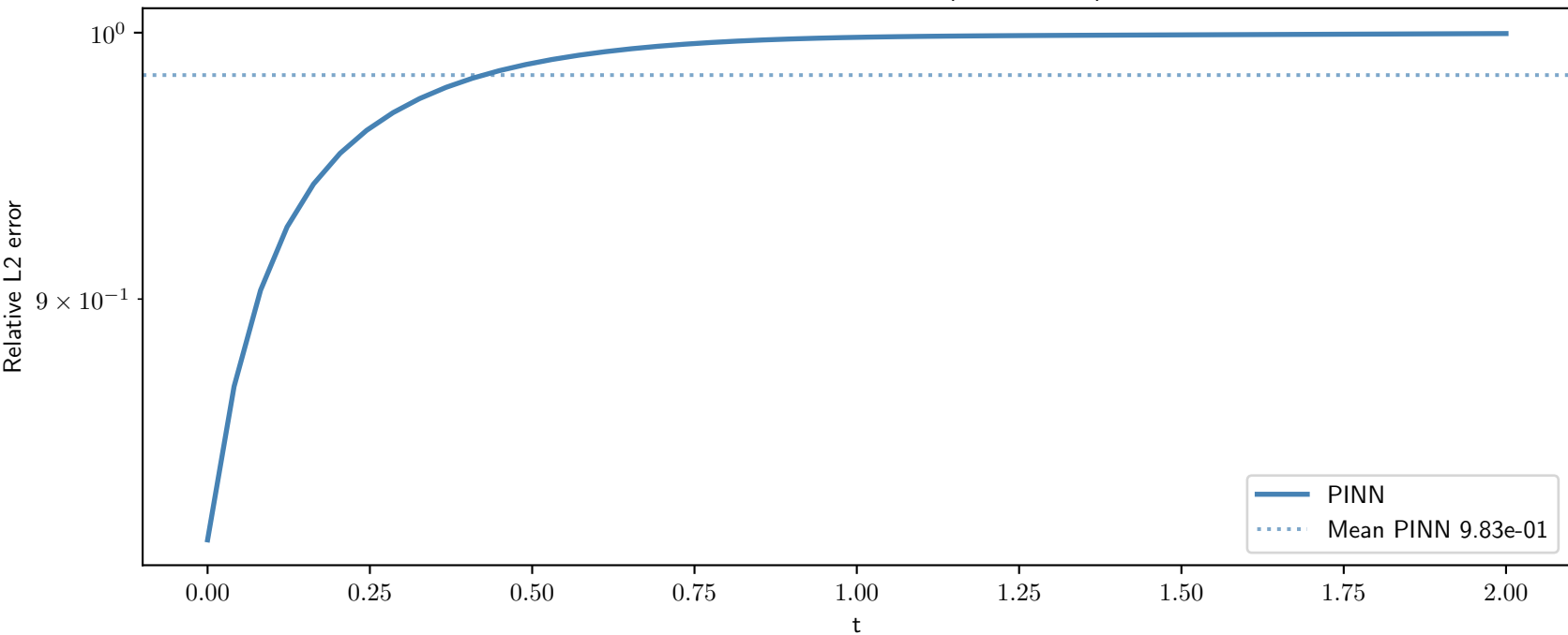
Relative L2 error over time ( \kappa = 0.0150 )
