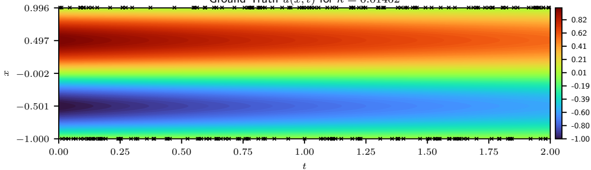
Ground Truth u(x, t) for \kappa = 0.01462
