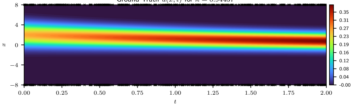
Ground Truth u(x, t) for \kappa = 0.94437
