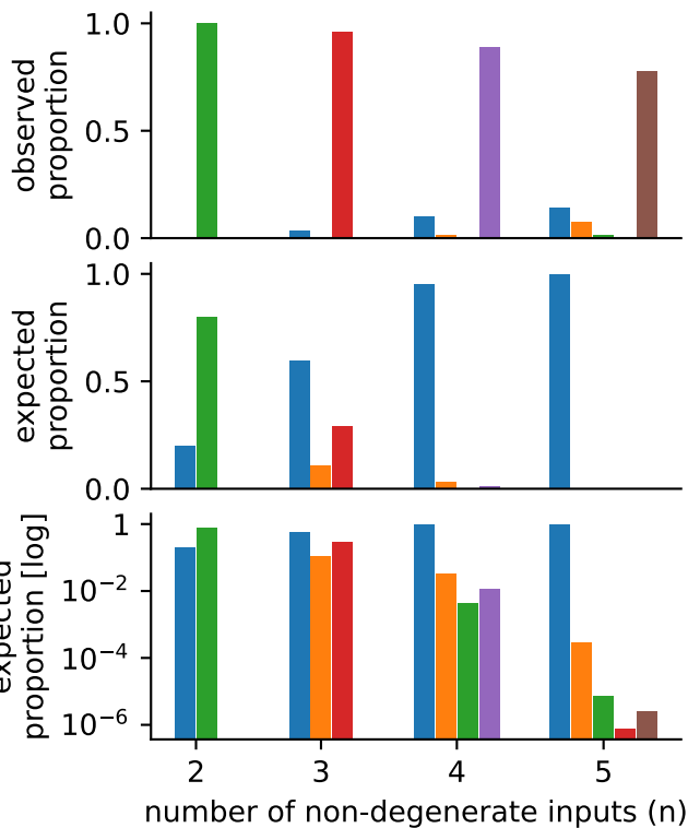
canalizing depth of non-degenerate Boolean function
