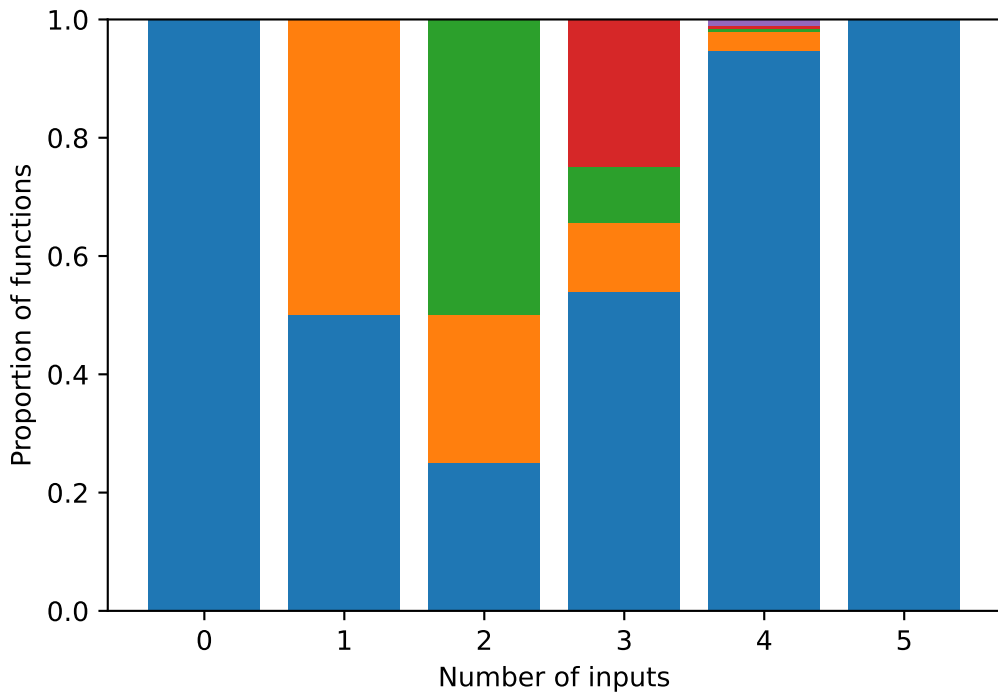
exact canalizing depth of Boolean function
