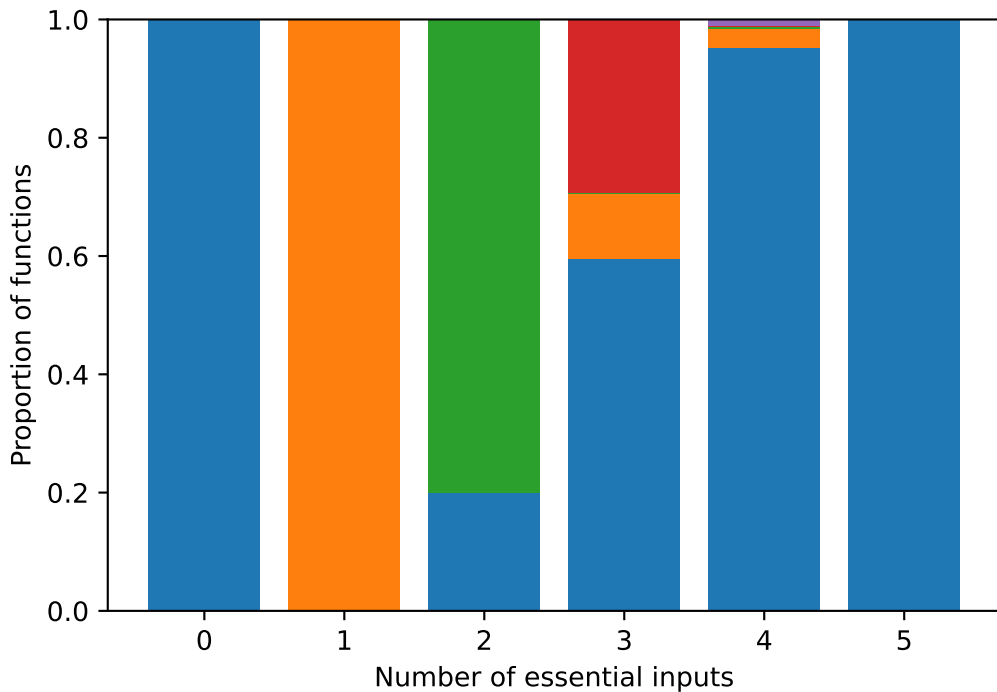
exact canalizing depth of non-degenerate Boolean function
