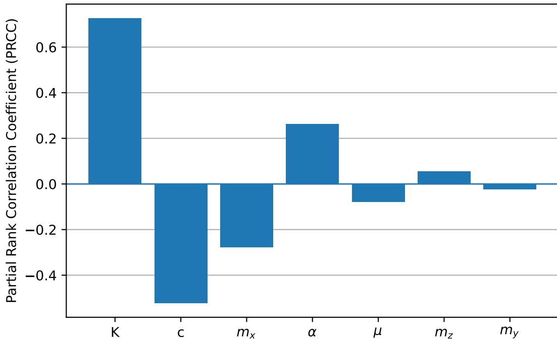
Final female abundance
