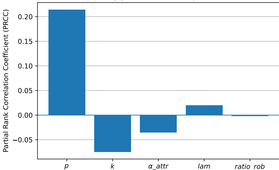
Strongly Connected Components
