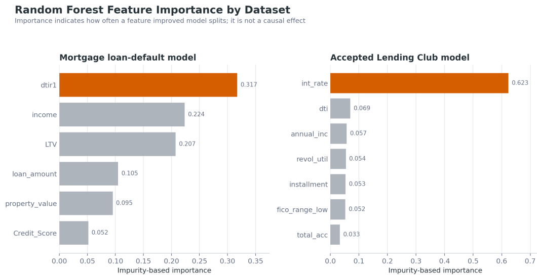
Figure 5. Random-forest impurity importance by dataset. Values describe model use, not causation.
