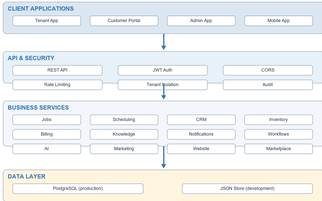
Figure 1. ServicePro platform architecture and request flow
