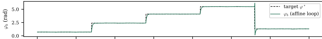
(a) MZM setpoint staircase across arbitrary points
