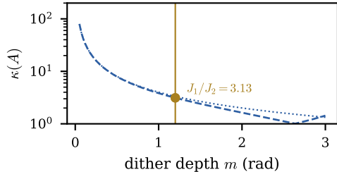
(c) \kappa(A) theory curve
