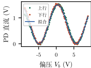
(a) 双向直流传递 V_\pi = 5.278 \text{ V}
